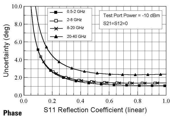
8722D with 85056A Calibration Kit
